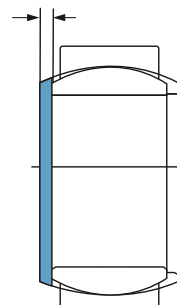
axial internal clearance 轴向内部游隙
